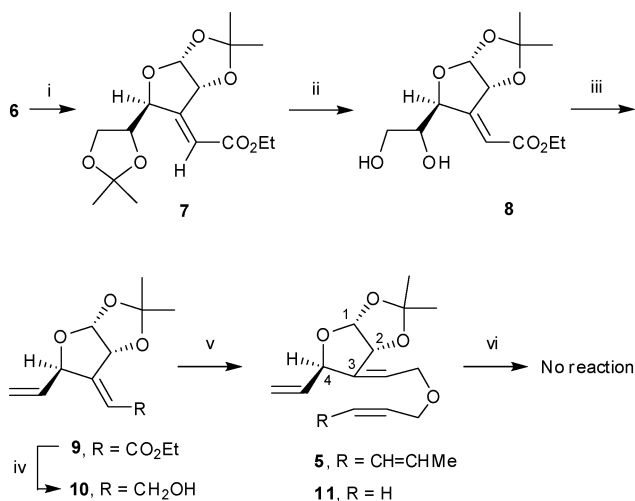
Scheme 2 Preparation of substrates 5 and 11 . Reagents and conditions: (i) (\text{EtO})_2\text{P}(\text{O})\text{CH}_2\text{CO}_2\text{Et} , NaH, THF, 0 °C, 0.5 h, 85% (1 : 4 E/Z separable mixture); (ii) AcOH–H 2 O (3 : 1), rt, 12 h, 88%; (iii) (a) MsCl, Et 3 N, DMAP (cat.), CH 2 Cl 2 , 0 °C → rt, 2 h; (b) NaI, DMF, 100 °C, 4 h, 80% two steps; (iv) DIBALH, CH 2 Cl 2 , –78 °C, 0.5 h, 96%; (v) NaH, THF–HMPA, reflux, sorbyl bromide for 5 , 85%; and allyl bromide for 11 , 90%; (vi) hν , Et 2 O, CuOTf (20 mol%), 6–12 h, no reaction.
