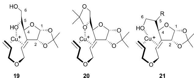
Fig. 2 Tri-co-ordinated Cu(I) complexes.
