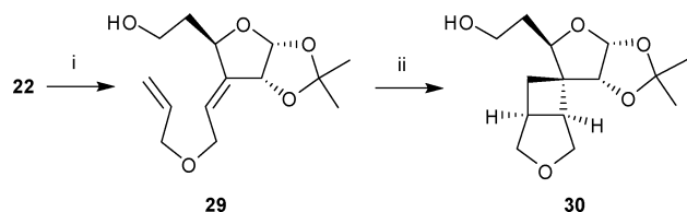
Scheme 5 Synthesis and photocycloaddition of substrate 29 . Reagents and conditions: (i) (a) Ph 3 PCH 2 OCH 3 Cl, KHMDS, THF, 0 °C; (b) 5% HCl, THF, 0 °C → rt, 15 min; (c) NaBH 4 , MeOH, 0 °C, 45% three steps; (ii) hv , Et 2 O, CuOTf (10 mol%), 3 h, 65%.
