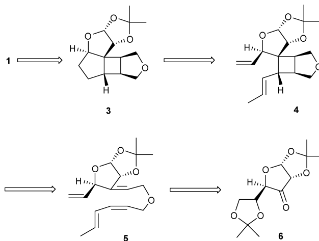
Scheme 1 Retrosynthesis.
