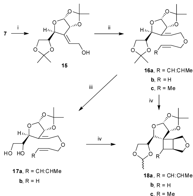
Scheme 3 Synthesis and [2 + 2] photocycloaddition of substrates 16a–c and 17a, b . Reagents and conditions: (i) DIBALH, CH 2 Cl 2 , –78 °C, 0.5 h, 96%; (ii) NaH, THF–HMPA, reflux, sorbyl bromide for 16a , 85%; allyl bromide for 16b , 90% and methylallyl bromide for 16c , 85%; (iii) AcOH–H 2 O (3 : 1), rt, 10 h, 75–80%; (iv) hν , Et 2 O, CuOTf (15–20 mol%), 4–4.5 h, 60–70%.
