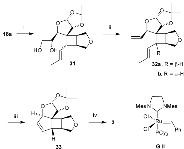
Scheme 6 Preparation of tetracycle 3 . Reagents and conditions: (i) DDQ (0.1 eqv.), CH 3 CN-H 2 O (9:1), 60 °C, 4 h, 80%; (ii) (a) MsCl, Et 3 N, DMAP (cat), CH 2 Cl 2 , quantitative; (b) NaI, DMF, 100 °C, 4 h, 80%; (iii) 8 mol% Grubbs' II, toluene, 100 °C, 4 h, 65% (96% based on the recovery of starting material as 32b ); (iv) H 2 , Pd-C, MeOH, 94%.
